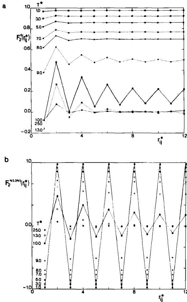
Figure 9. The dependence of the anisotropic second rank orientational correlation functions on the scaled separation, r_{ij}^* , for a selection of the scaled temperatures, T^* , studied in the simulation: (a) F_2^0(r_{ij}^*) and (b) F_2^{\pi/3, 2\pi/3}(r_{ij}^*) .
