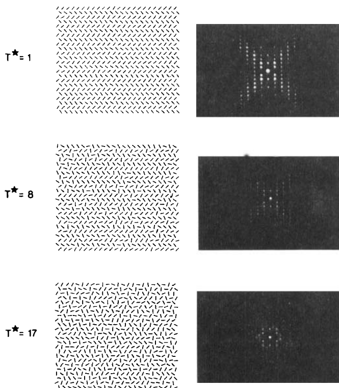
Figure 10. Typical configurations for the smectic E phase ( T^* = 1 and 8) and for the smectic B phase ( T^* = 17 ) together with their optical transforms.
